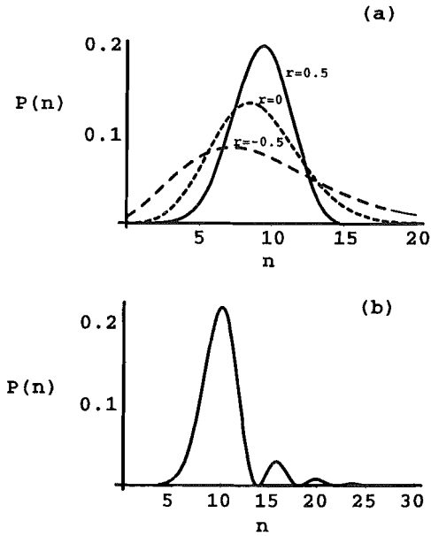
Fig. 2.4 Photon number distribution for a squeezed state |\alpha, r\rangle : (a) \alpha = 3 , r = 0, 0.5, -0.5 , (b) \alpha = 3 , r = 1.0
